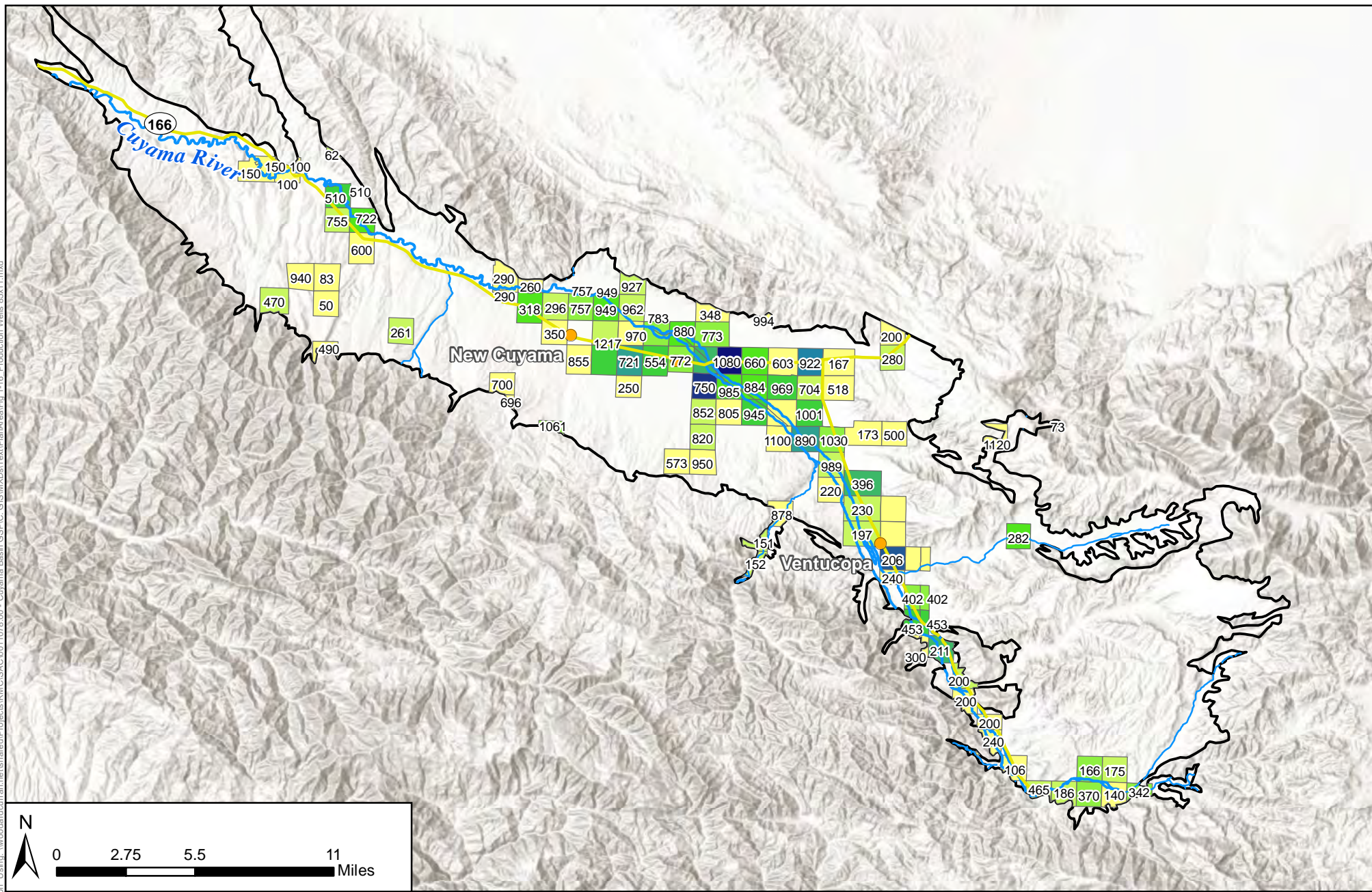
Figure 1-16 - Production Well Density and Average Depths Cuyama Basin Groundwater Sustainability Agency Cuyama Valley Groundwater Basin Groundwater Sustainability Plan December 2019
