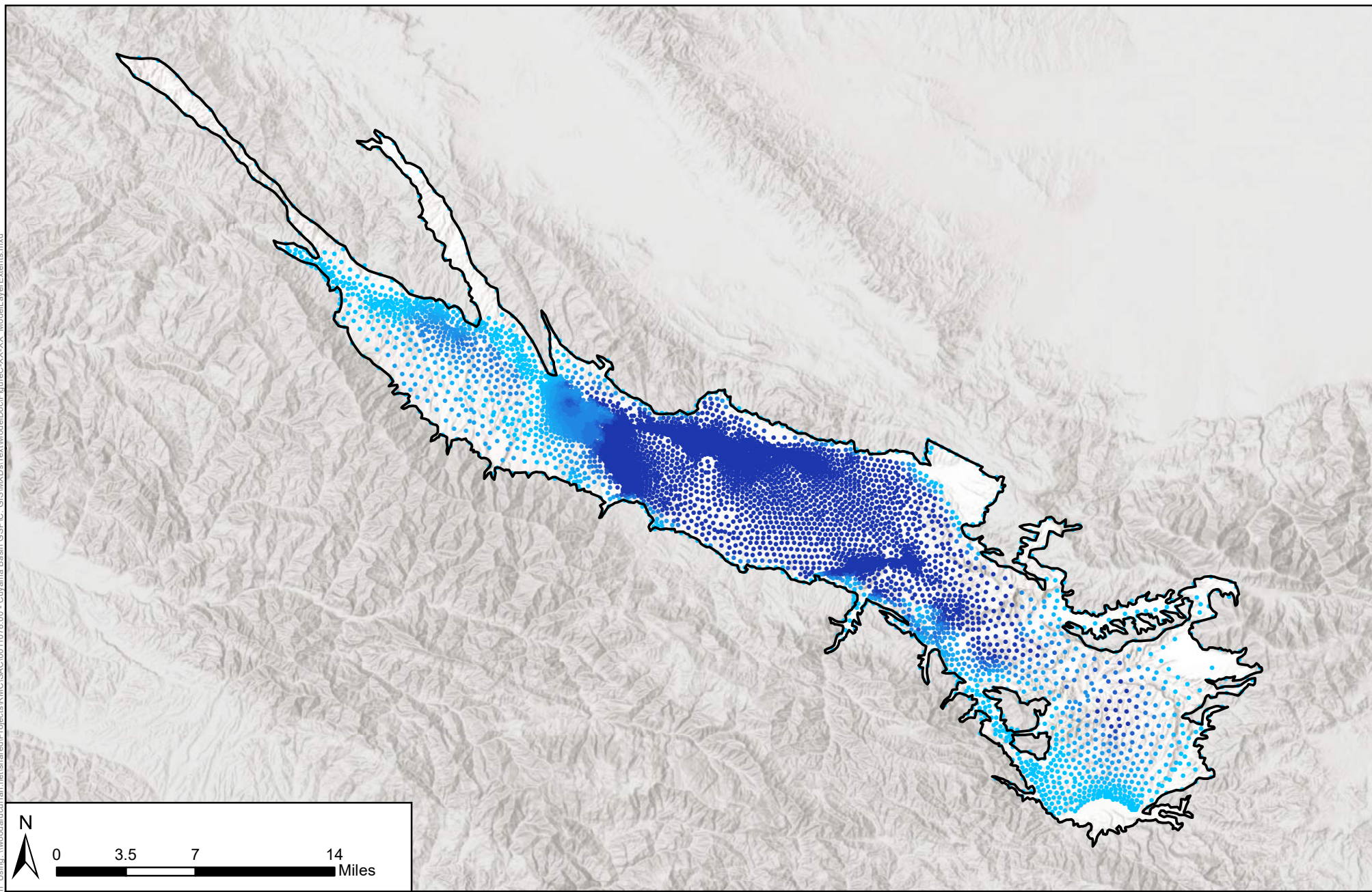
Figure C-14 - CBWRM Layer 3 Extent and Thickness Cuyama Basin Groundwater Sustainability Agency Cuyama Valley Groundwater Basin Groundwater Sustainability Plan June 2019
