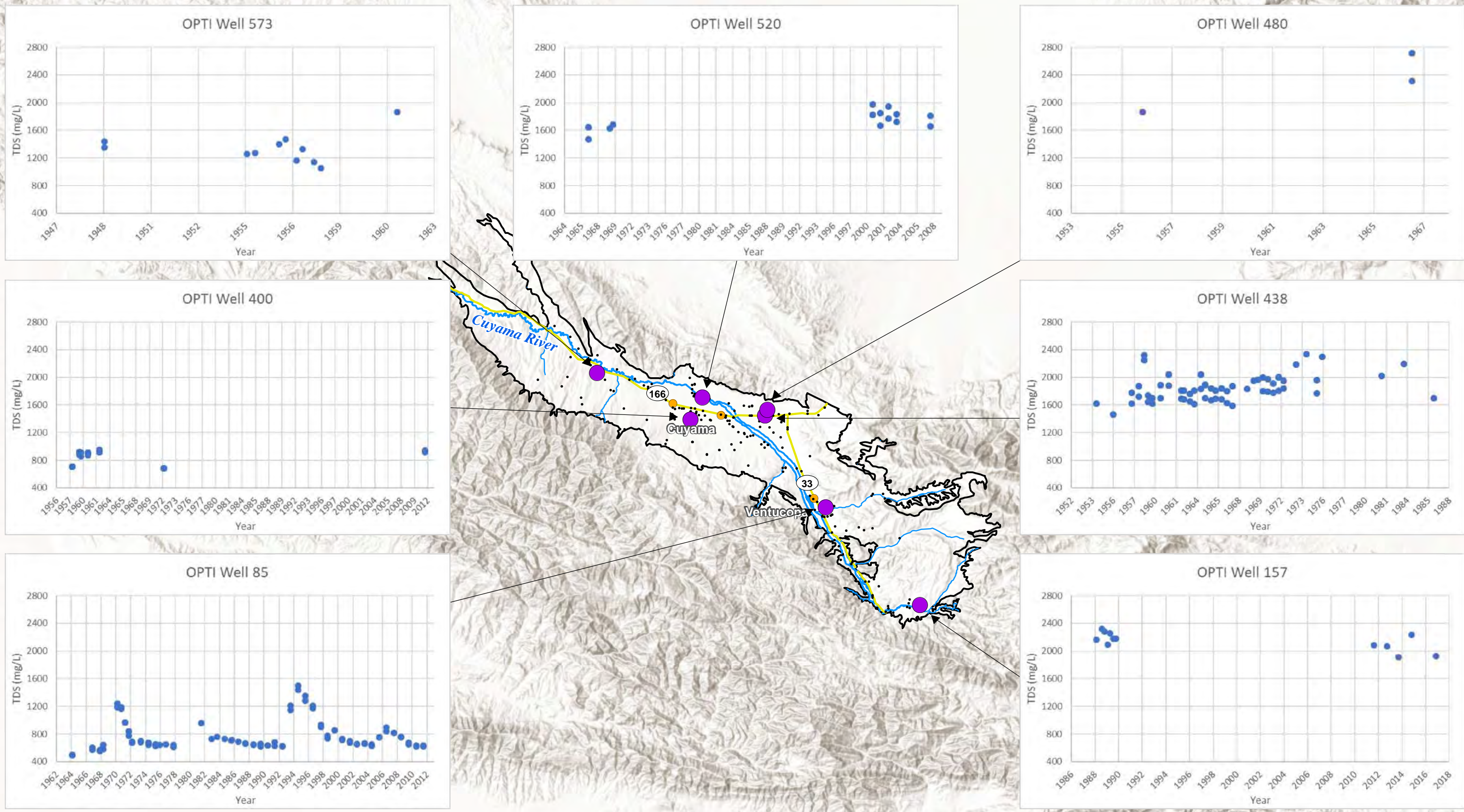
Figure 2-54: Cuyama Groundwater Basin Historic TDS Levels in Selected Wells Cuyama Basin Groundwater Sustainability Agency Cuyama Valley Groundwater Basin Groundwater Sustainability Plan December 2019
