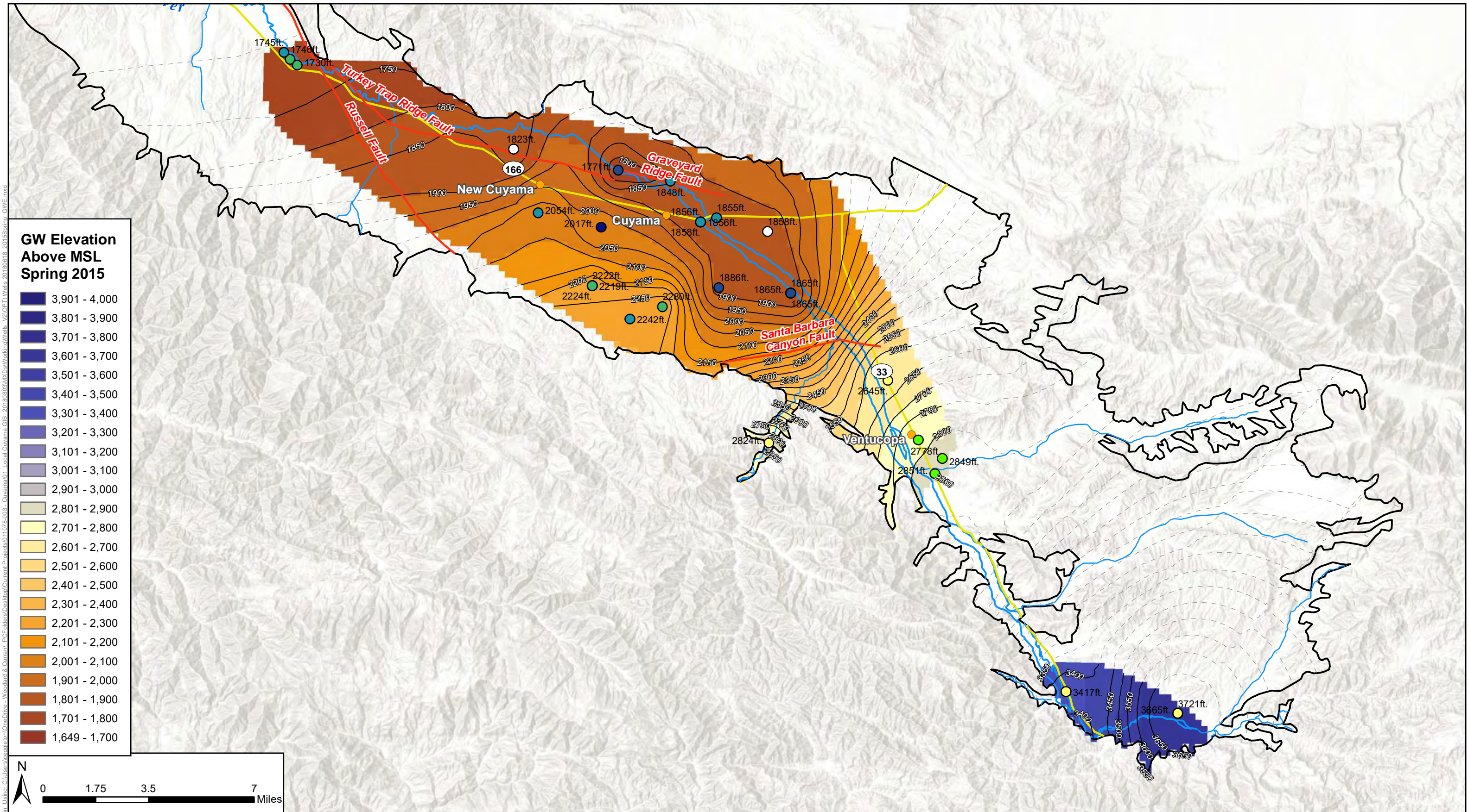
Figure 2-45: Spring 2015 Groundwater Elevation Cuyama Basin Groundwater Sustainability Agency Cuyama Valley Groundwater Basin Groundwater Sustainability Plan September 2019
