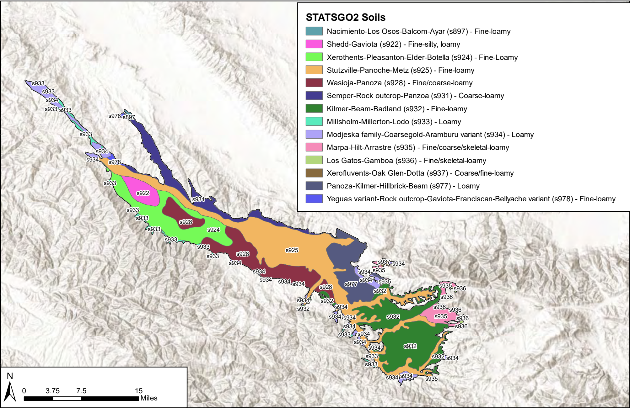
Figure 2-19: Soils Cuyama Basin Groundwater Sustainability Agency Cuyama Valley Groundwater Basin Groundwater Sustainability Plan December 2019
