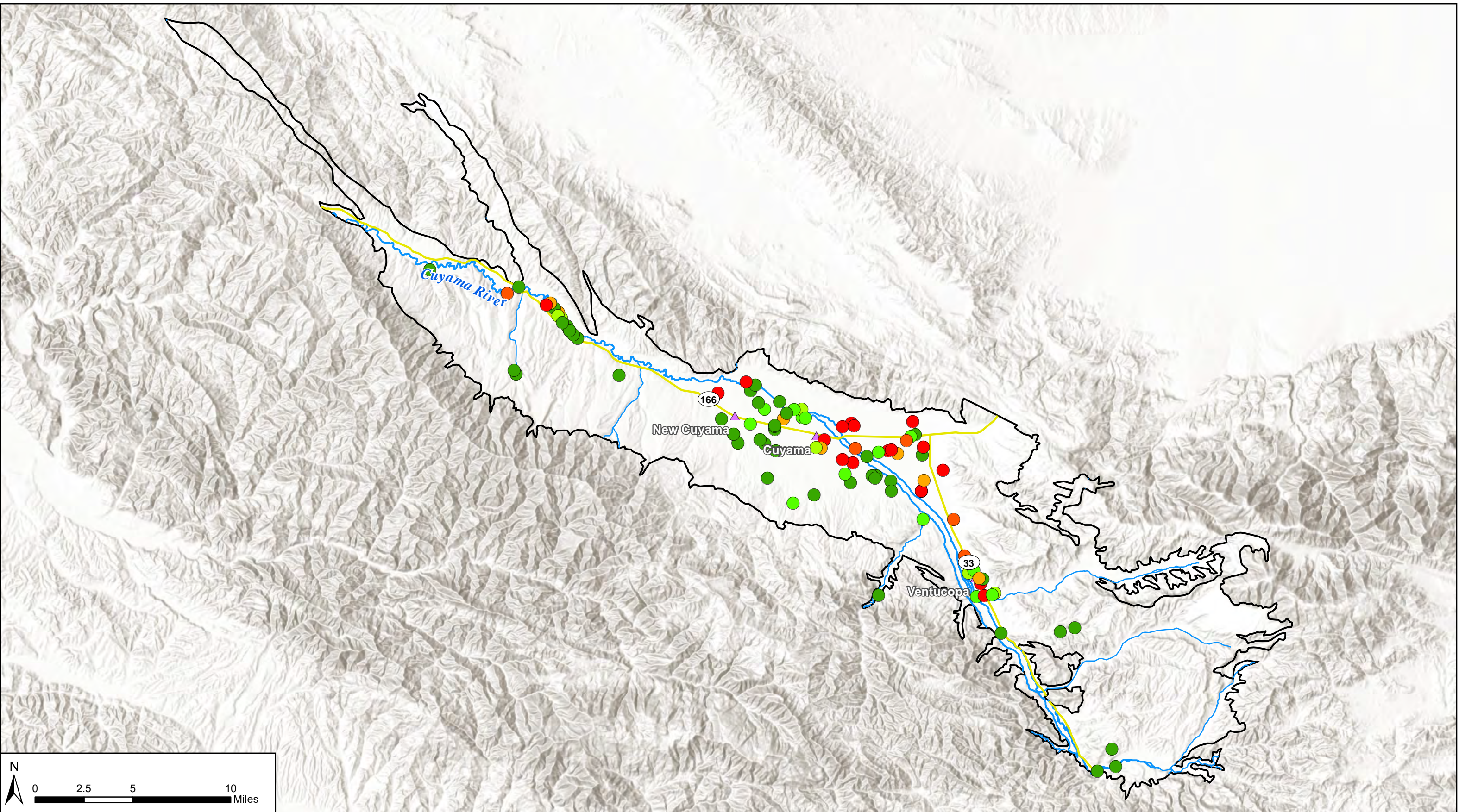
Figure 2-79: 2010-2020 Average Well Measurements of Nitrate (NO3) as Nitrogen Cuyama Basin Groundwater Sustainability Agency Cuyama Valley Groundwater Basin Groundwater Sustainability Plan October 2021
