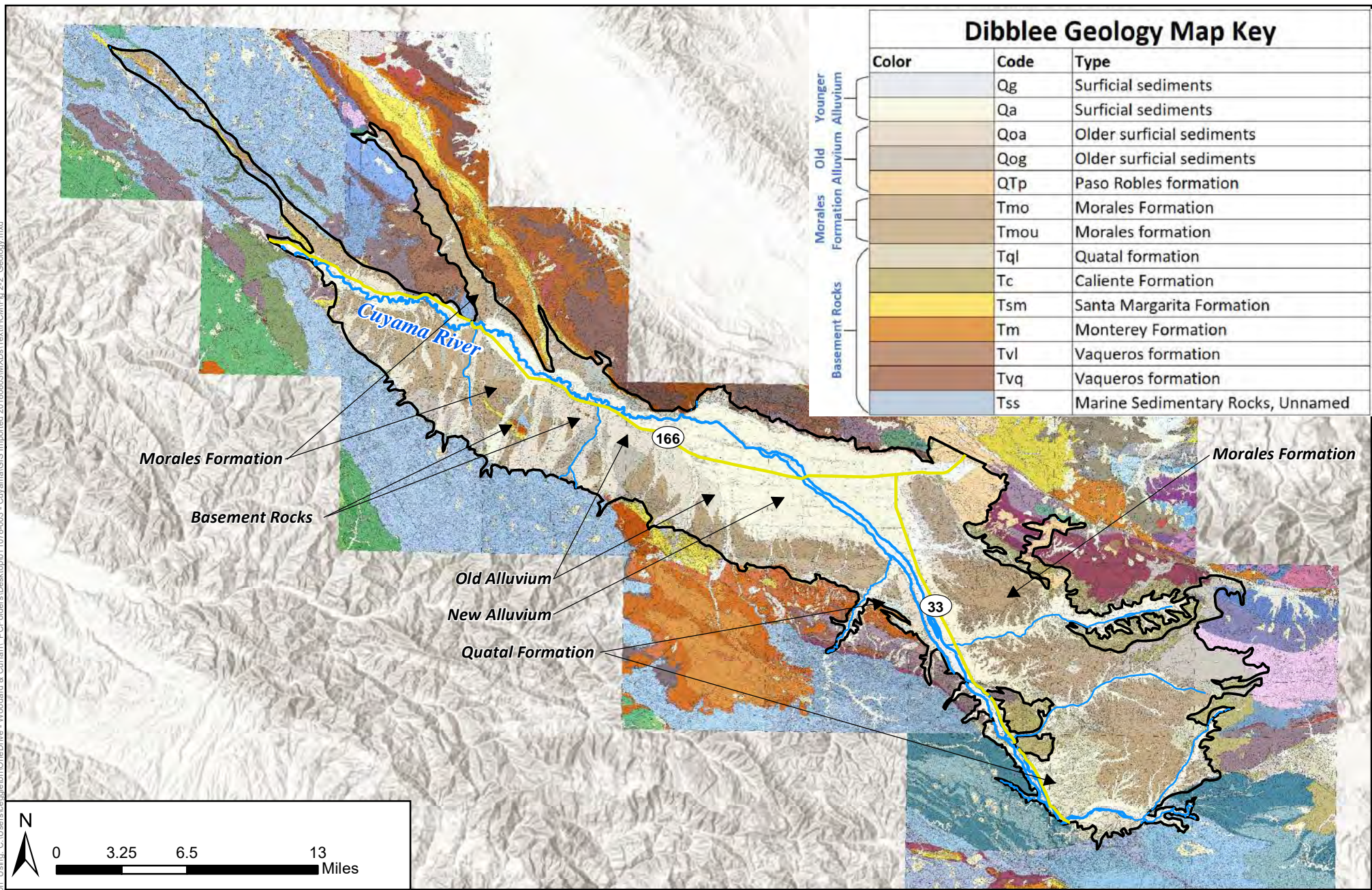
Figure 2-2: Geologic Map
