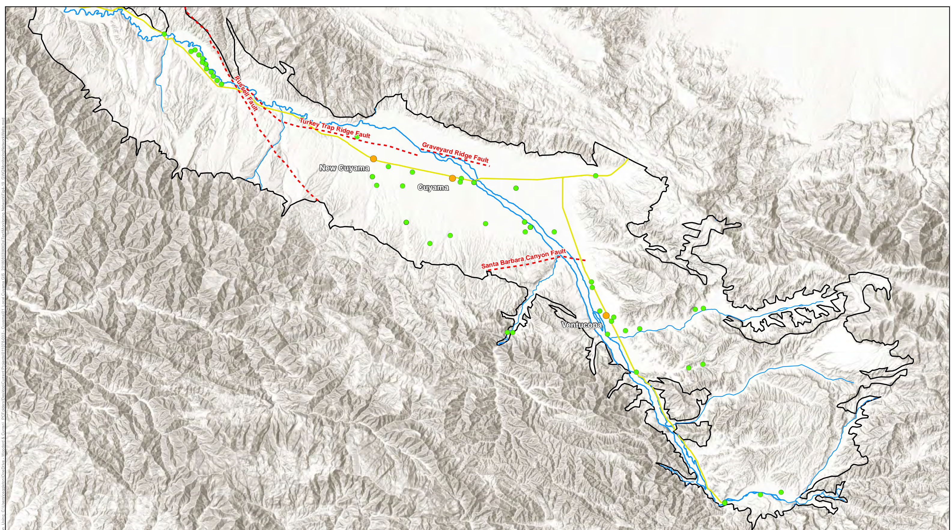
Figure 4-20: Cuyama GW Basin Groundwater Quality Monitoring Network Wells Cuyama Basin Groundwater Sustainability Agency Cuyama Valley Groundwater Basin Groundwater Sustainability Plan December 2019
